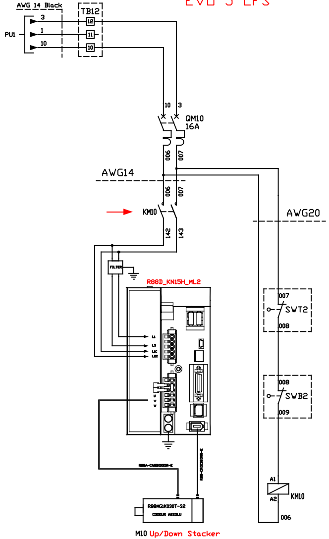
M10 Up/Down Stacker
