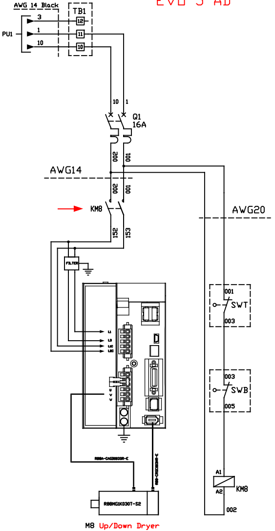
M8 Up/Down Dryer
